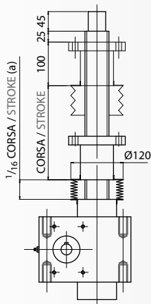
VITE ROTANTE / ROTATING SCREW VR
