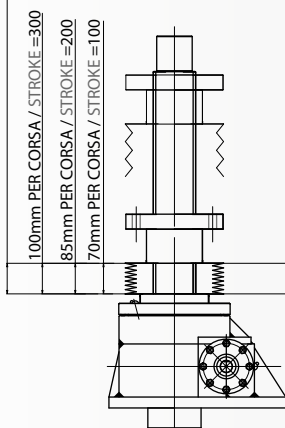
VITE ROTANTE / ROTATING SCREW VR
