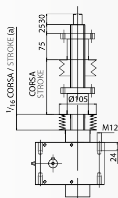
VITE ROTANTE / ROTATING SCREW VR
