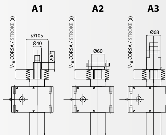
VITE TRASLANTE / TRAVELLING SCREW VT
